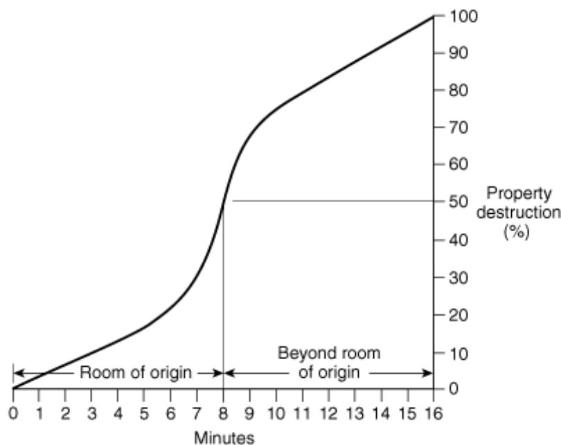
FIGURE A.5.2.2.2.1 Fire Propagation Curve.
